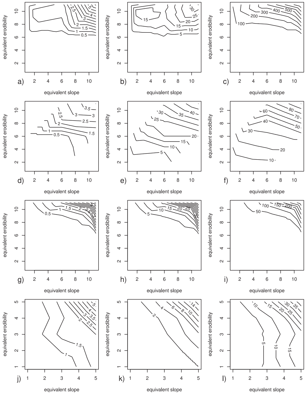
Figure 7. Sensitivity maps for (a–c) MHYDAS, (d–f) STREAM, (g–i) PESERA, and (j–l) MESALES in spatially homogeneous configurations. Precipitation and runoff conditions increase from left to right for each model, except for MESALES, which is mapped in a median runoff condition but for increasing precipitation. Soil loss isovalues are in t\ ha^{-1}\ event^{-1} for MHYDAS and STREAM and in t\ ha^{-1}\ yr^{-1} for PESERA and MESALES.
