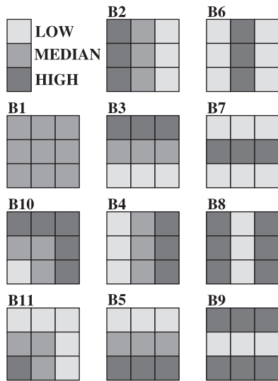
Figure 2. Spatially distributed B configurations. Light, medium, and dark gray cells receive values of erosion parameters associated with low, median, and high efficiency with respect to soil loss, respectively.
