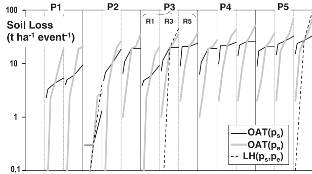
(b) STREAM - same key as (a)
