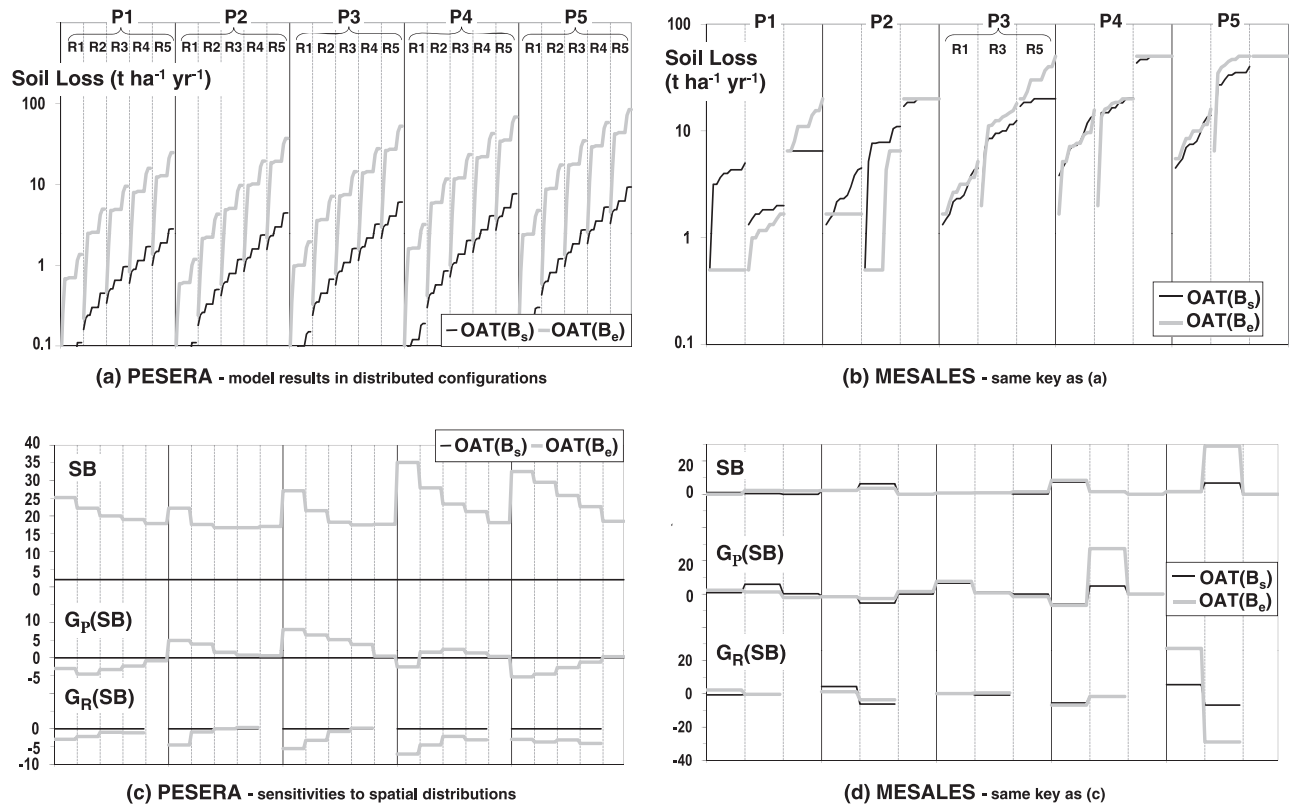
Figure 9. Dashboards representing soil loss, dispersion SB, and variations in SB for (a, c) PESERA and (b, d) MESALES under all combinations of precipitation P and runoff conditions R for OAT screenings (Figure 4b) involving spatial distributions of the equivalent slope B_s or erodibility B_e .
