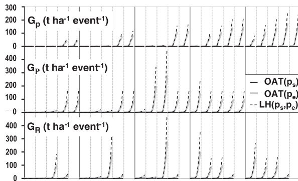
(c) MHYDAS - sensitivities in homogeneous configurations
