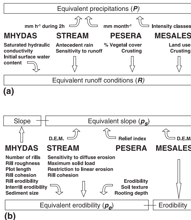
Figure 3. Innate entries of each model chosen for definition of (a) equivalent control hydrological conditions and (b) equivalent “descriptive” parameters of slope and erodibility. Slope appears as such in the innate parameterization of MHYDAS, as does erodibility in MESALES.
