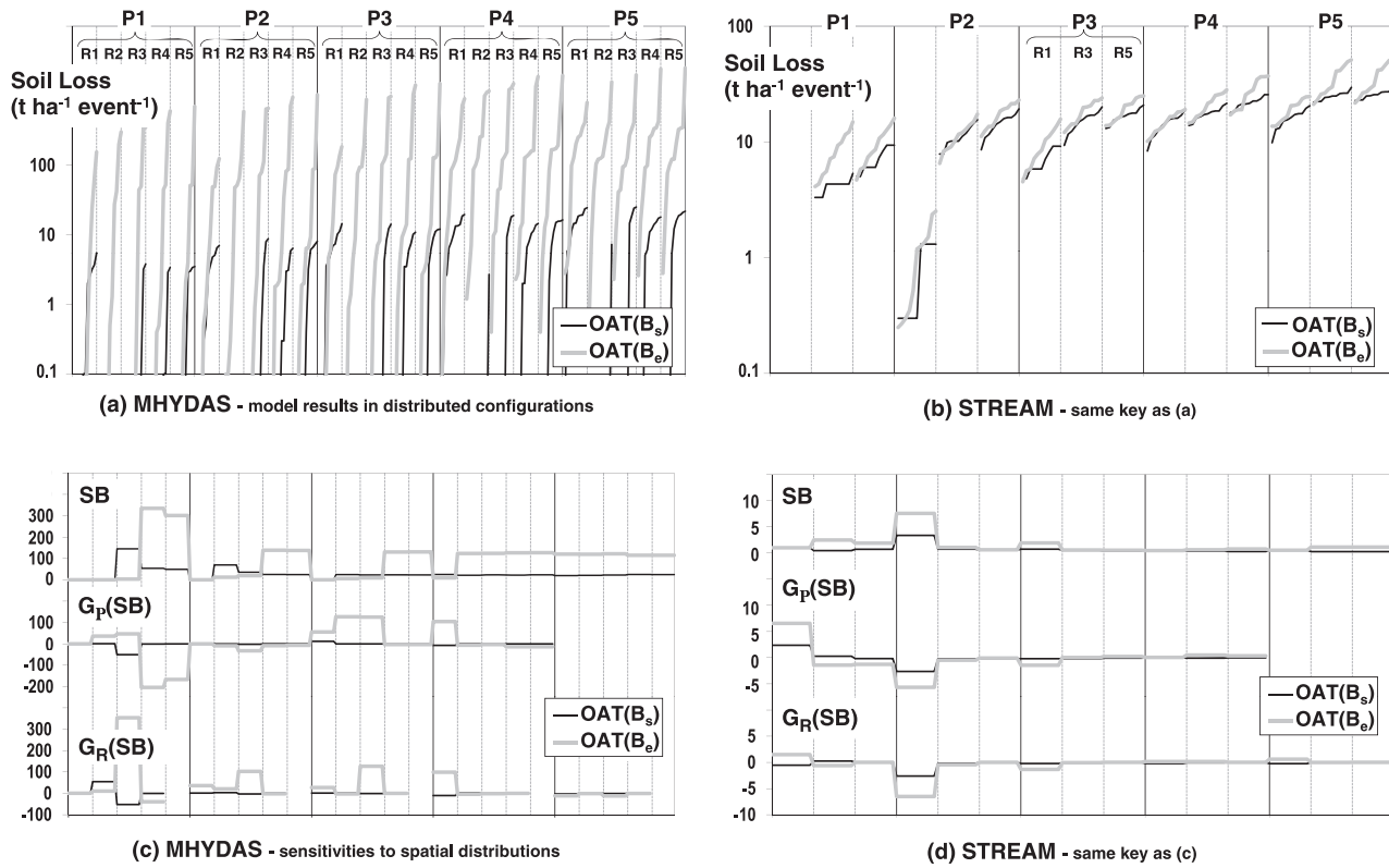
Figure 8. Dashboards representing soil loss, dispersion SB, and variations in SB for (a, c) MHYDAS and (b, d) STREAM under all combinations of precipitation P and runoff conditions R for OAT screenings (Figure 4b) involving spatial distributions of the equivalent slope B_s or erodibility B_e .
