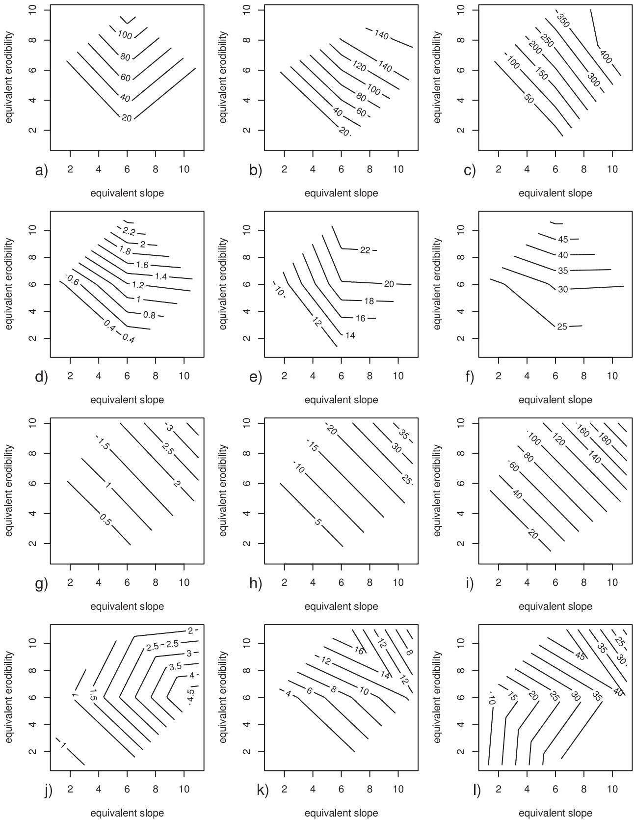
Figure 10. Sensitivity maps for (a–c) MHYDAS, (d–f) STREAM, (g–i) PESERA, and (j–l) MESALES in spatially distributed configurations. Precipitation and runoff conditions increase from left to right for each model, except for MESALES, which is mapped in a median runoff condition but for increasing precipitation. Soil loss isovalues are in t\ ha^{-1}\ event^{-1} for MHYDAS and STREAM and in t\ ha^{-1}\ yr^{-1} for PESERA and MESALES.
