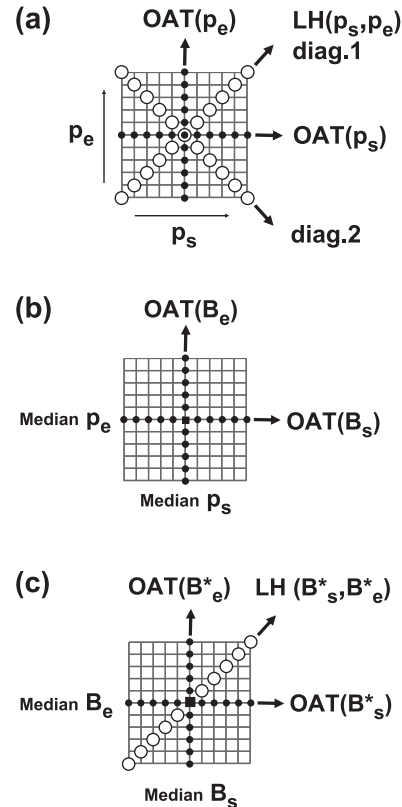
Figure 4. Screening stages and strategies, involving tests on the equivalent slope p_s and equivalent erodibility p_e in (a) spatially homogeneous or (b, c) distributed configurations, where equivalent parameters are denoted B_s and B_e , respectively. One-at-a-time (OAT) and Latin hypercube (LH) explorations are assembled into sensitivity maps.
