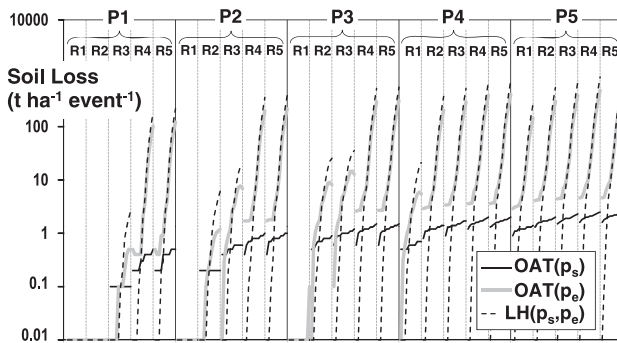
(a) MHYDAS - model results in homogeneous configurations
