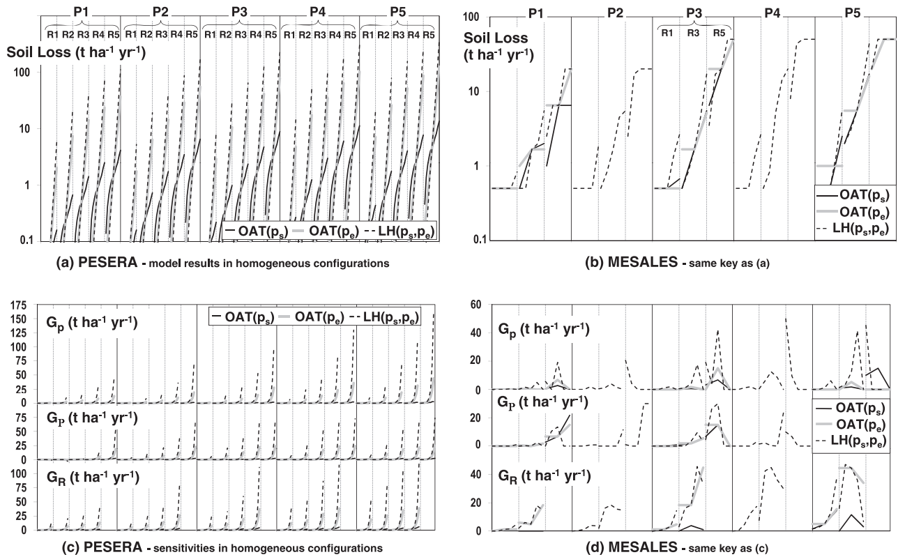
Figure 6. Dashboards representing soil loss and sensitivity results for (a, c) PESERA and (b, d) MESALES under all combinations of precipitation P and runoff conditions R for OAT and LH screenings involving spatially homogeneous values of the equivalent slope p_s and/or erodibility p_e .
