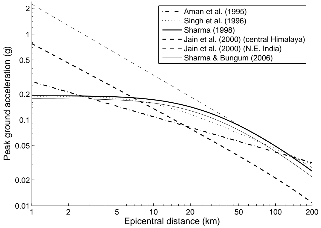
Figure 1: Comparison of horizontal PGA predicted by various empirical ground-motion models developed using Indian strong-motion data for an M_w 6.0 [ m_b 5.6 , using the magnitude-conversion formula of Castellaro et al. (2006): m_b = (M_w + 1.272)/1.291 ] earthquake with a focal depth of 10 km.
