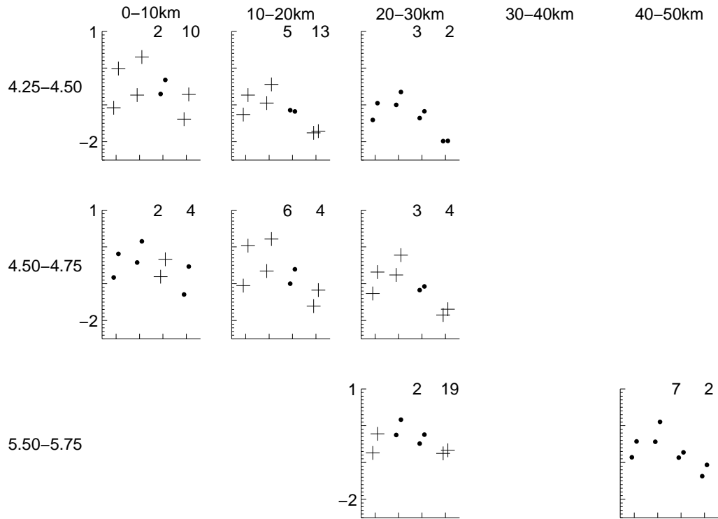
Figure 7: Graphs for each bin where analysis of variance was performed to compare ground motions in Molise and Umbria-Marche. Each small graph displays the means of the transformed ground motions for each of the four strong-motion intensity measures considered (the first two points are PGA, the second two points are SA at 0.2s, the third two points are SA at 0.5s and the final two points are SA at 1.0s). The ordinate of the small graphs is logarithm of acceleration in m/s^2 . Therefore they can be thought of as response spectra with only four ordinates. The left point in each pair is for Molise and the right point is for Umbria-Marche. If the difference in means was found to be significant at the 5% significance level using the F-test then the marker is a cross rather than a dot. The two numbers in the top right corner are the total number of records in the bin from each region (the left number is for Molise and the right number is for Umbria-Marche). The small graphs are arranged in an overall plot showing the magnitude (on the y-axis) and distance (on the x-axis) ranges of the bins. Since no comparisons could be performed due to insufficient data, the magnitude range between 4.75 and 5.50 is not shown.
