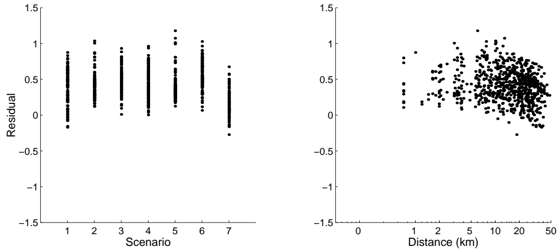
Figure 5: Residuals between the empirical estimates and the simulations for horizontal PGV with respect to scenario and distance to the seismogenic rupture.
