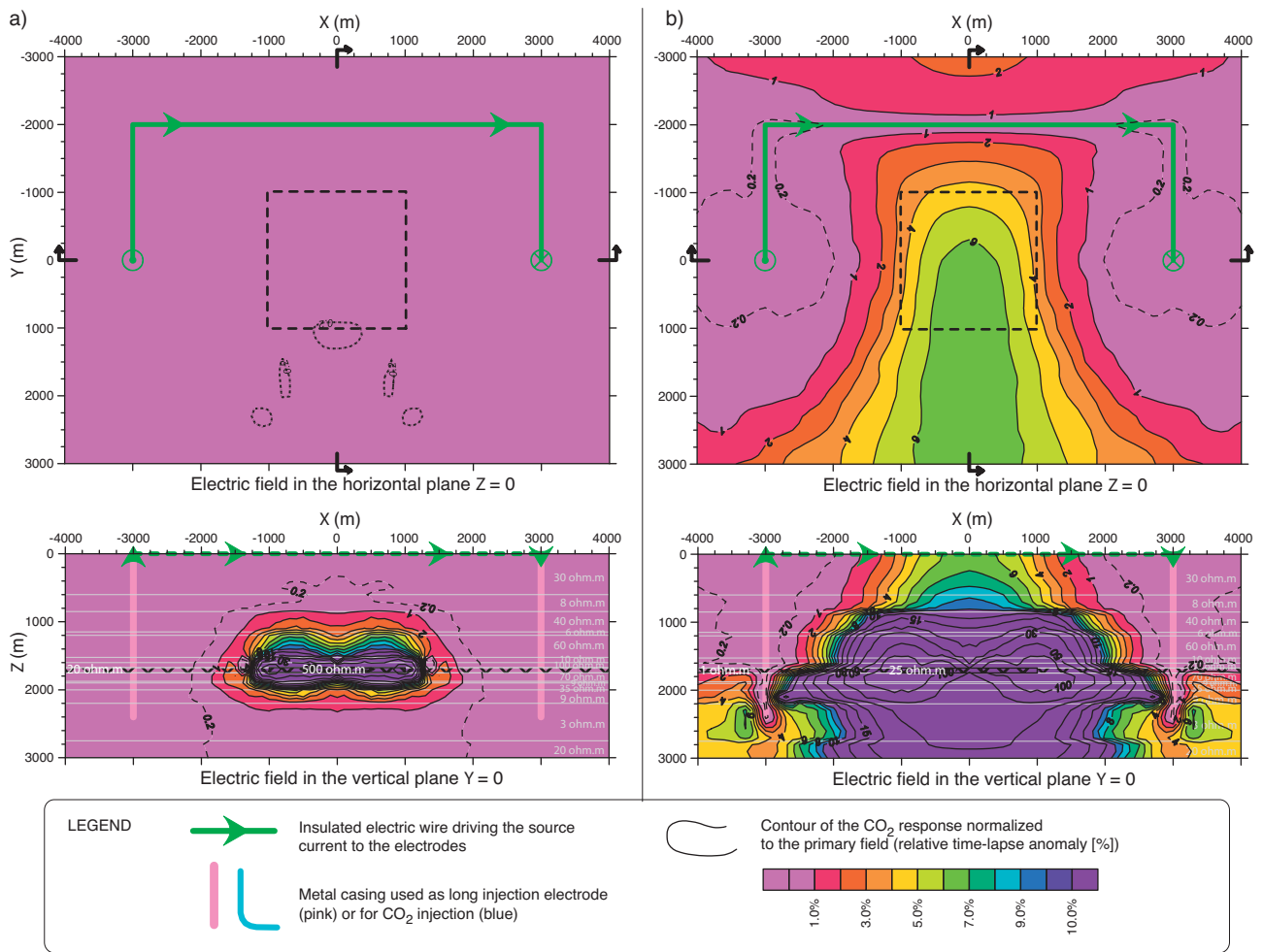
Figure 9 Relative time-lapse electric response (major axis) from the CO 2 bubble defined in Figure 5 for a LEMAM injection at 0.5 Hz for two variants of the reservoir layer: a) for a realistic reservoir of 20 ohm.m; b) for a favourable reservoir of 1 ohm.m.
