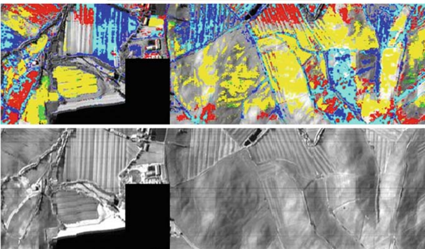
447 448 Fig. 7.4 ULM facility and resulting images: one based on Spectral Angle Mapper (SAM) classifica- 449 tion; the second based on SWIR data where absorption bands of mineral clays (2.0–2.4 \mu\text{m} ) 450 are present (Univ. Firenze). Red : calcite, green : chlorite, yellow : illite, blue : illite-smectite, cyan : smectite
