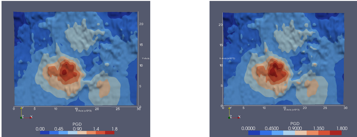
Figure 14: Peak Ground Displacements during the linear (left) and nonlinear (right) simulations for the 0.6 Hz mesh.
