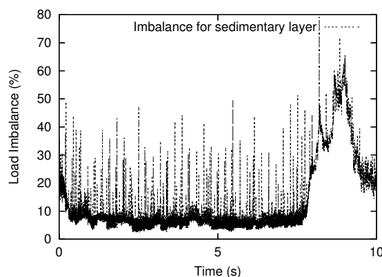
Figure 10: Variation with time of the imbalance induced by the variation of the numerical cost in the sedimentary layer with a non linear rheology.
