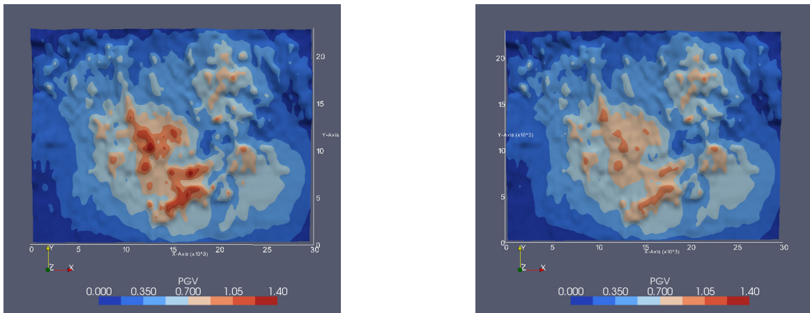
Figure 15: Peak Ground Velocities during the linear (left) and the nonlinear (right) simulations for the 0.6 Hz mesh.
