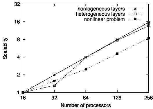
Figure 9: Impact of the numerical behavior of our algorithm on load balancing in the case of the 0.5 Hz mesh.
