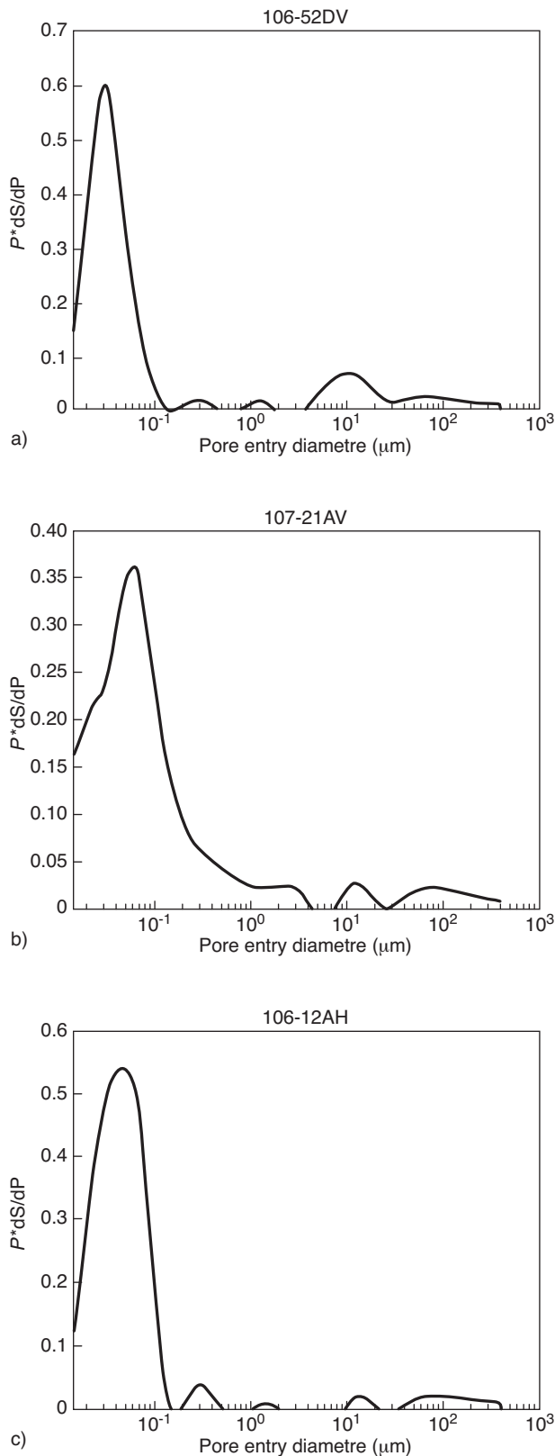
Figure 7 Pore throat size distribution for the 3 different facies from High Pressure Mercury Injection (HPMI).
