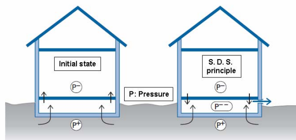
Figure 4: Soil Depressurization System S.D.S. principle: the air flow direction between the basement and the indoor environment is inverted by the pressure decrease at the interface (denoted P^{--} ), hence preventing the gaseous pollutant advective upwards migration (adapted from Collignan and Sullerot, 2008)
