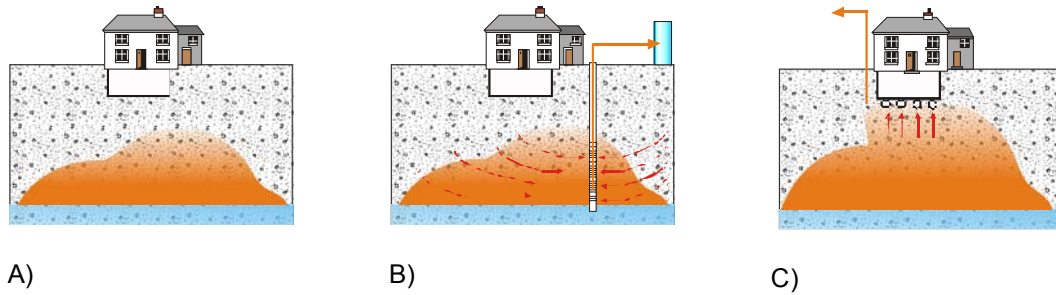
Figure 2: intervention strategy for managing the transfer of CO 2 within the vadose zone : A) monitored natural attenuation ; B) active extraction techniques such as SVE; C) protection of targets through techniques aiming at stopping the vertical migration of CO 2
