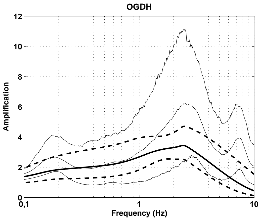
Figure 14: Comparison between the mean amplification curve and its 10 and 90% confidence limits computed using the one-quarter wavelength method (thick lines) and the mean amplification curve and its 10 and 90% confidence limits computed using the Haskell-Thompson method (thin lines) for the OGDH station. The profiles simulated using the Monte Carlo technique developed in this article are used for both computations.
