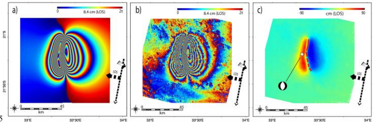
Figure 7: a) Interferogram simulation obtained using the inverted parameters. One fringe corresponds to 8.4 cm in LOS. The approximate locations of the modelled fault surfaces are shown. b) Interferogram 2004/04/06 – 2006/05/07 unwrapped taking into account the simulation and rewrapped for visualisation purposes (one fringe corresponds to 8.4 cm in LOS) c) Interferogram 2004/04/06 – 2006/05/07 geocoded and unwrapped taking into account the simulation. Values in rad. The fault trace derived from post-seismic deformation is shown.
