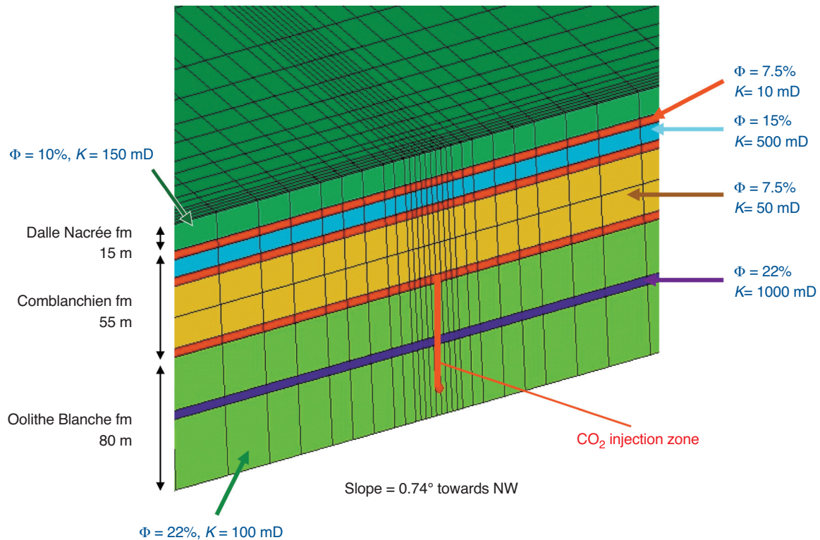
Figure 17 Part of the 3-D grid used to calculate CO 2 -water movements in the Dogger formations. Relatively thin layers were considered within the formations, to represent specific rock types actually observed in the field, either in the Oolithe Blanche Formation (very conductive layers are known from the area exploited for geothermal energy, in the central part of Paris Basin), or in the Comblanchien Formation (dolomite-rich, highly permeable tops of sequence were studied from SMB and from outcrops).
