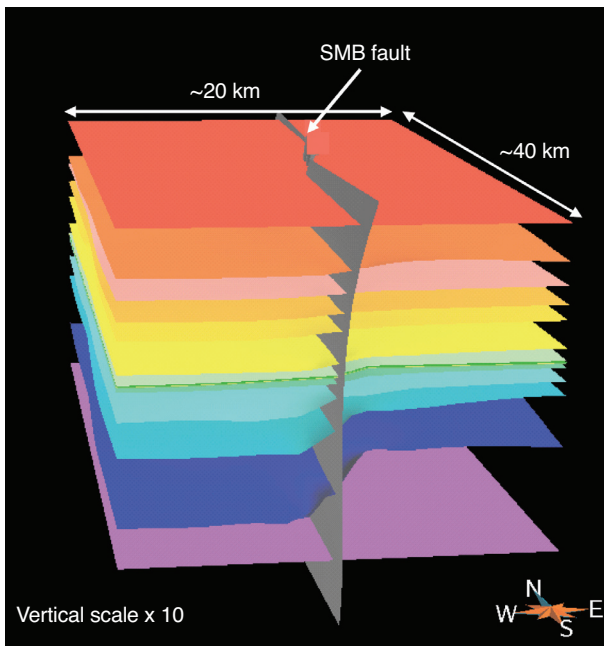
Figure 16 The 3-D numerical block representing the earth's model of the SMB site. The modelled layers are listed in Vidal-Gilbert et al. (2009).
