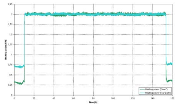
Figure 11: Thermal power injected in the soil by the two control loops during the 6 days thermal response test
