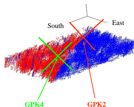
Figure 14: Compartmentalisation of the fracture density and hydraulic properties – View of the pipe conductivities.
