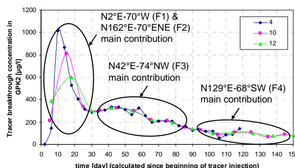
Figure 11: Contribution of each fracture set to the GPK2 tracer breakthrough.
