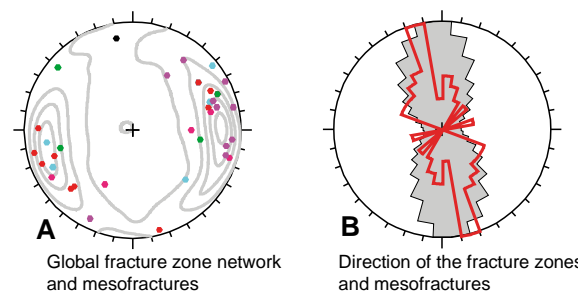
Figure 12: Synthesis of the orientation of fractures at different scales in the Soultz granite. A- Poles of fracture zones from the different wells (Green: EPS1, pink: GPK1, blue: GPK2, red: GPK3,
